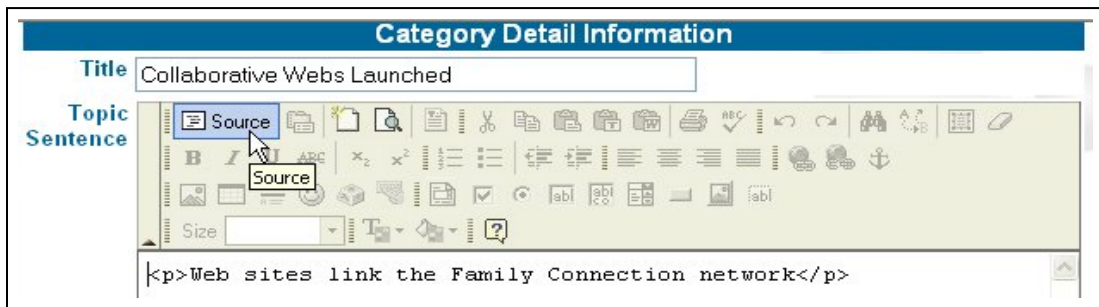
Figure 3.5 Source Code
